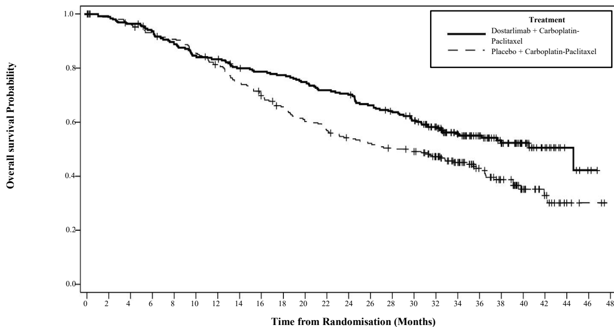
Figure 2. Kaplan-Meier curve of overall survival in all patients (overall population) with EC (RUBY study)
